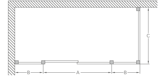
Sliding door with in-line and side panel
