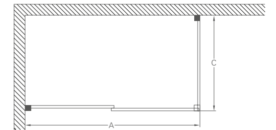
Sliding door with side panel
